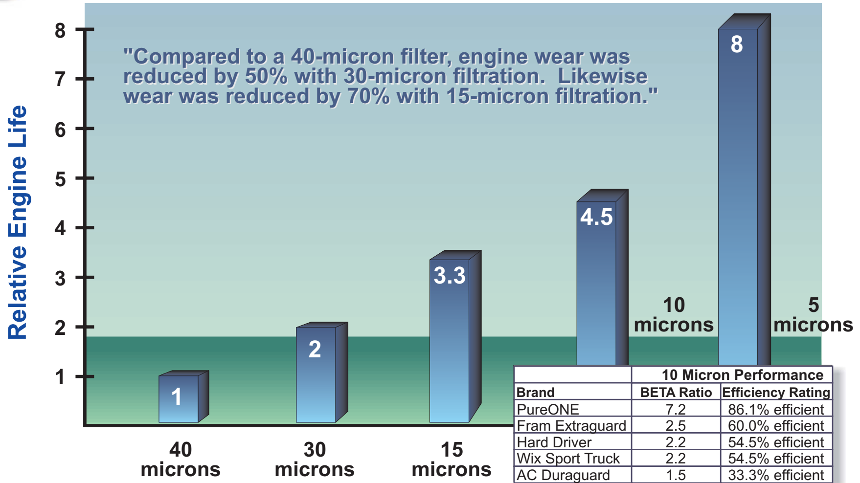
Performance of Crankcase Filter
